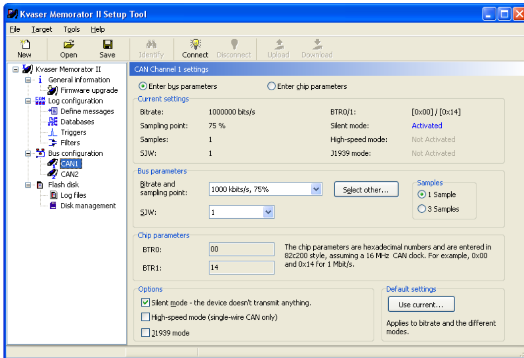
Figure 20. Bus configuration.
