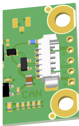
Figure 3: The CAN connector.
