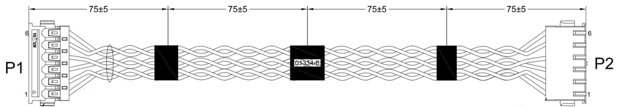
Figure 8: PCB-to-PCB cabling.
