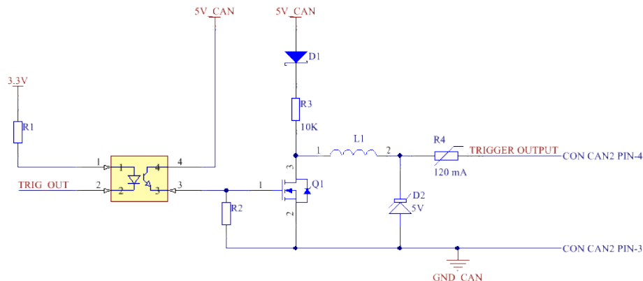
Figure 12: The External trigger output inside the Kvaser Memorator Pro 5xHS.
