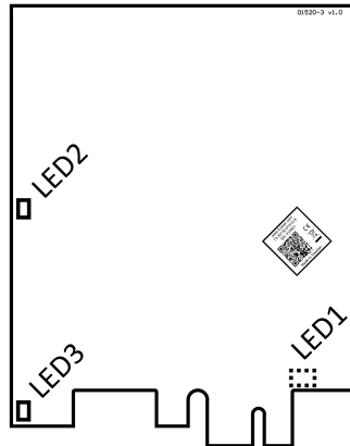
Figure 3: LEDs on the Kvaser PCIe 8xCAN.
