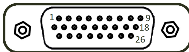
Figure 4: The male 26 pin HD D-SUB connector pin numbers
