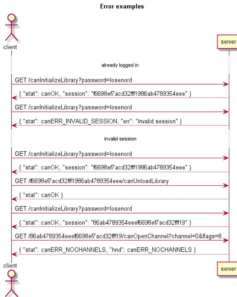
Figure 8: Error examples
