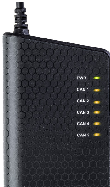
Figure 4: LEDs on the Kvaser USBcan Pro 5xHS.
